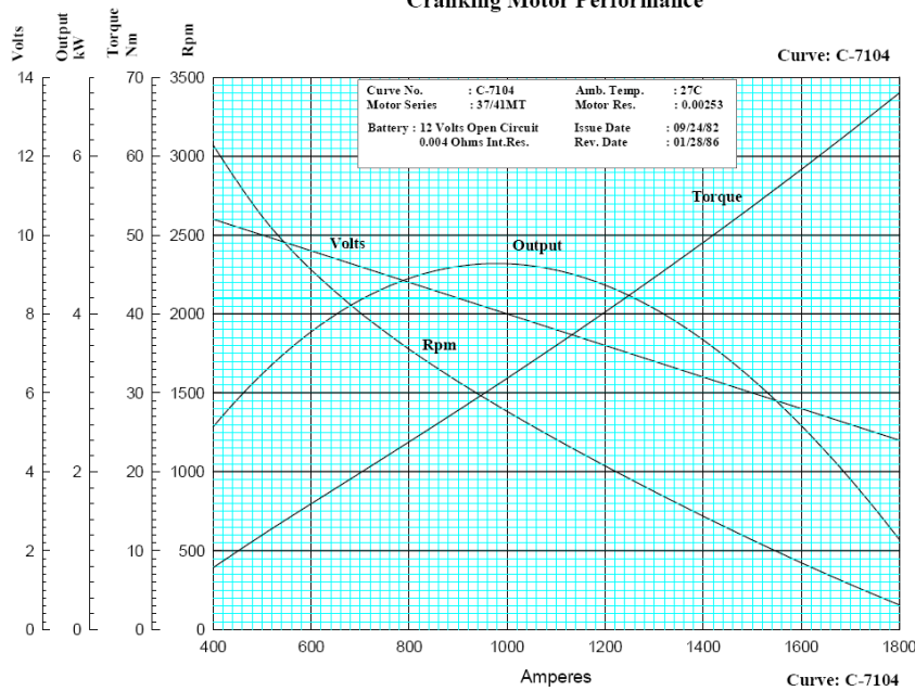
Cranking Motor Performance
