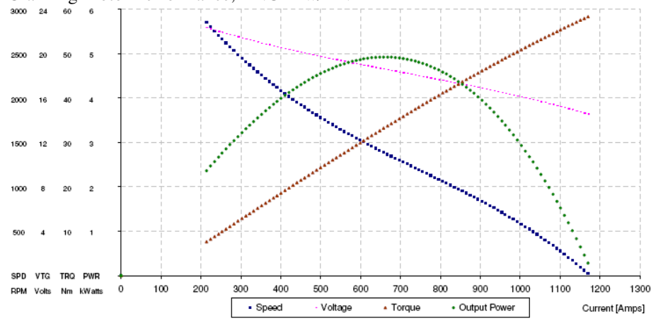
Cranking Motor Performance, BNG 4kw/24V
